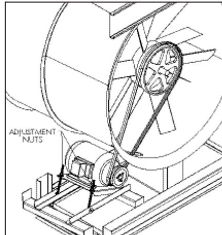
Figure 7 – PM Style Motor Adjustment
