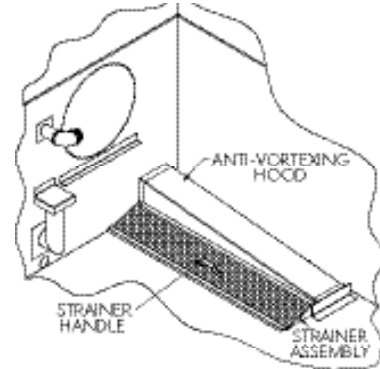
Figure 11 – LSWE/LSC-E/PMC-E Strainer Assembly
