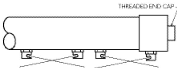
Figure 17 – Proper Water Diffuser Orientation (2A Nozzles) ESW4 Models
