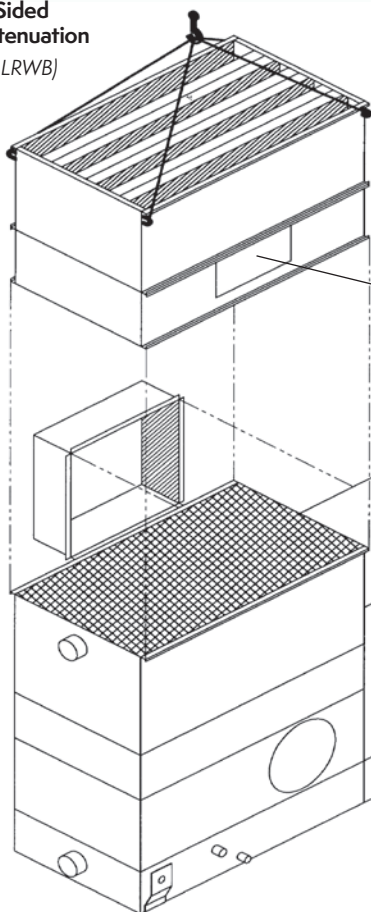
Drift Eliminator and Water Distribution Access Panel
