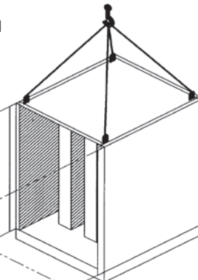
Drift Eliminator and Water Distribution Access Panel
