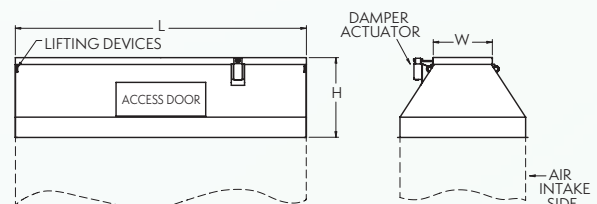
Tapered Discharge Hood (See page 22 for dimensions)
