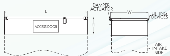
Straight-Sided Discharge Hood (See page 22 for dimensions)
