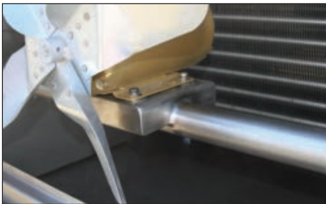
Fully Welded Stainless Pipe Motor Mount with "Spacer" Between the Motor and the Support for Complete Cleaning
