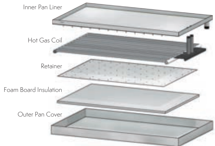
Hot Gas Drain Pan
