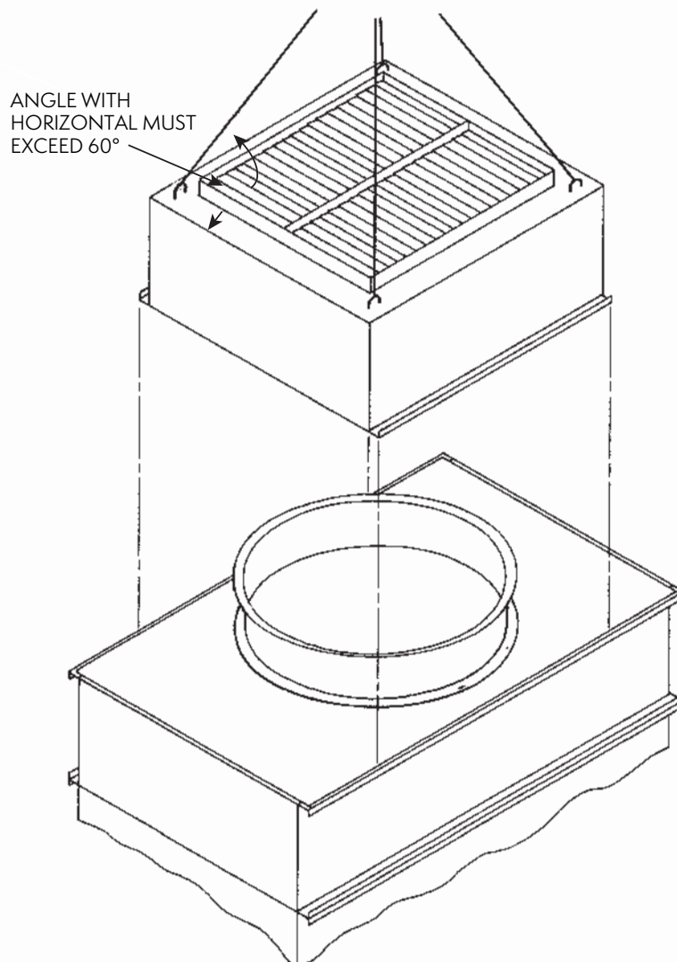
Figure 31 – Mating Discharge Hood Damper Section to Coil/Fan Section
