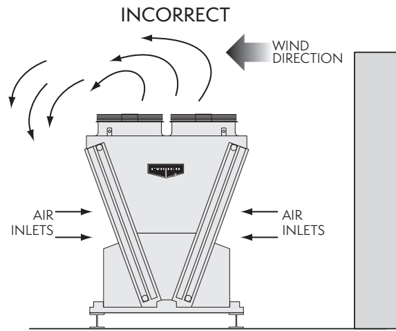
Figure 2 - Effect of Wind Directed Toward Surrounding Structure when Top of Unit is Lower Than Adjacent Structure
