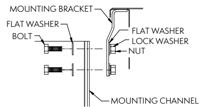
Figure 21 – Mounting Channel Installation
