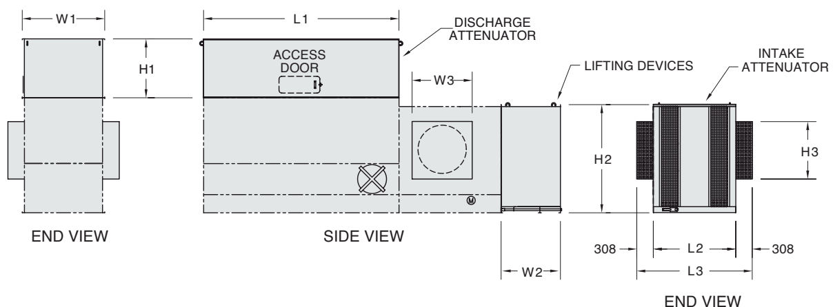
LRC Attenuation
